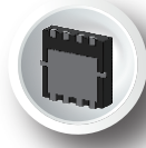
PDFN3030 3.10*3.30*0.75mm
