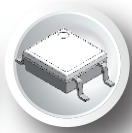
MFP-4L 4.40*3.60*1.90mm 3.75 kVrms
