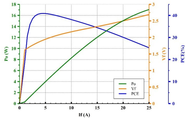
0.1ms pulse width and 1% duty cycle
