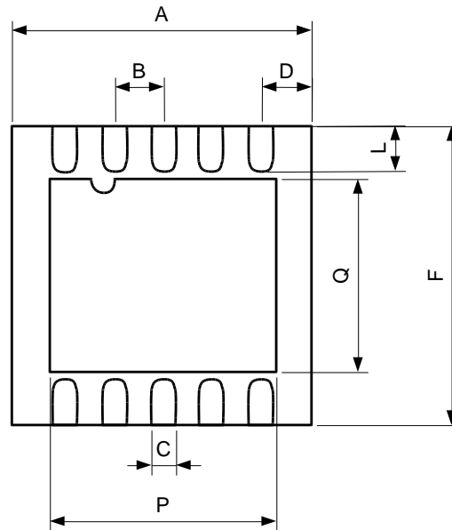
Figure 12.4 DFN-10 Package Dimensions (bottom view)
