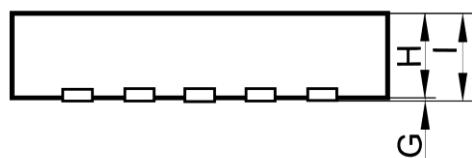
Figure 12.5 DFN-10 Package Dimensions (side)
