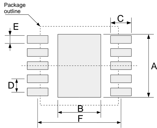
Figure 12.6 Recommended DFN-10 Landing Dimensions
