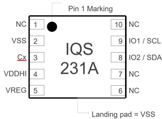
Figure 2-4 IQS231AB 10-pin DFN Package
