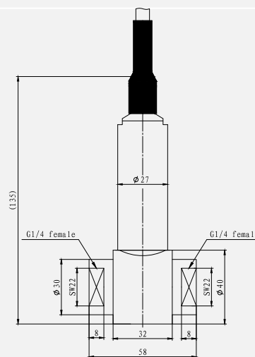
Cable Type (B2)
