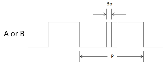
Figure 29: ABZ Jitter
