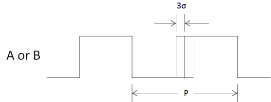
Figure 28: ABZ Jitter
