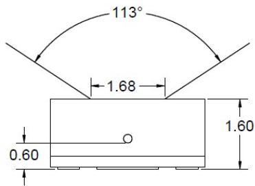
Side-X view
