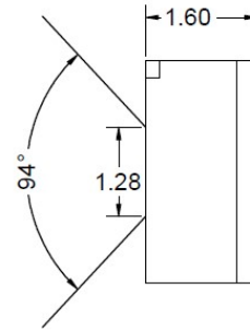
Side-Y view
