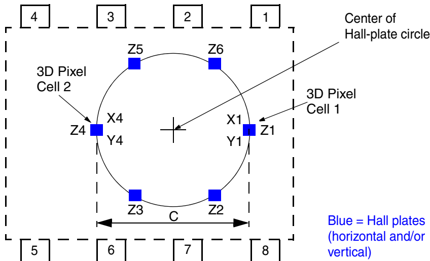
Fig. 3–1: Hall-plate position definition for HAL 3960
