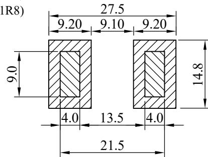
( PCB Pattern )
