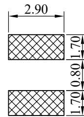
( PCB Pattern )
