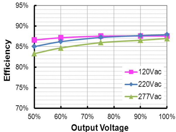
EUC-026S070SVM0004( I_o=500mA ) Efficiency vs. Output Voltage
