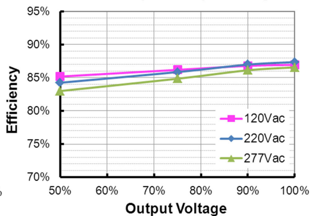
EUC-026S070SVM( I_o=700mA ) Efficiency vs. Output Voltage
