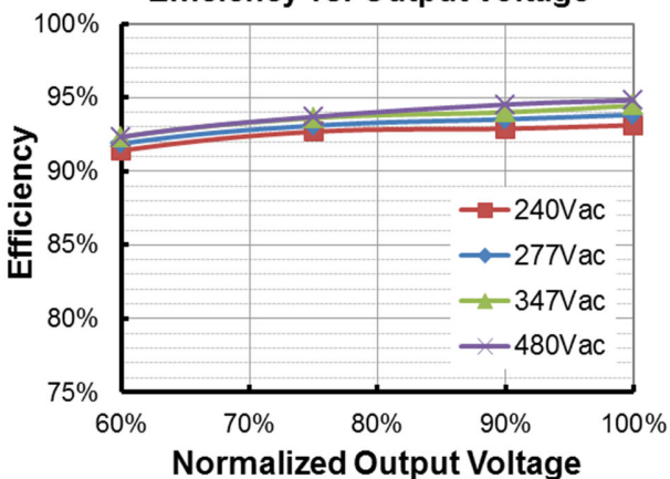
EFD-1K2S740DV( I_o=5920mA ) Efficiency vs. Output Voltage
