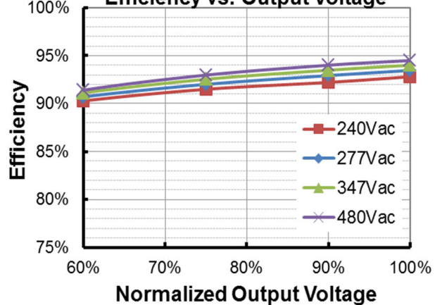
EFD-1K2S740DV( I_o=7400mA ) Efficiency vs. Output Voltage
