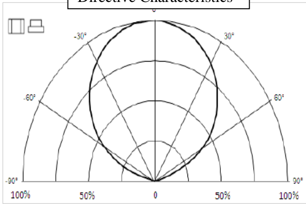
Directive Characteristics
