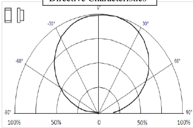
Directive Characteristics
