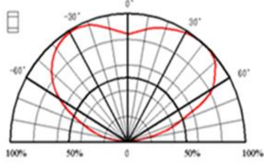
Directive Characteristics
