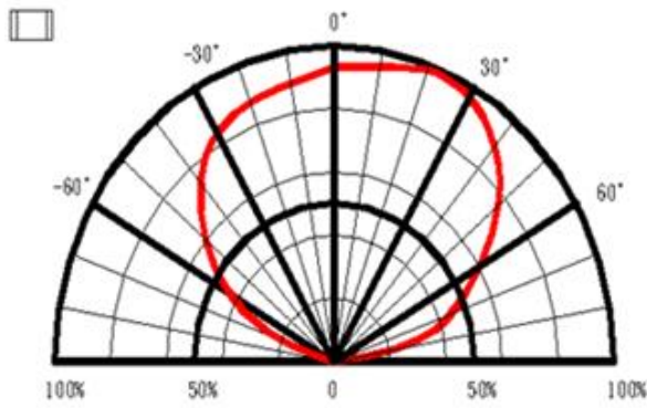
Directive Characteristics
