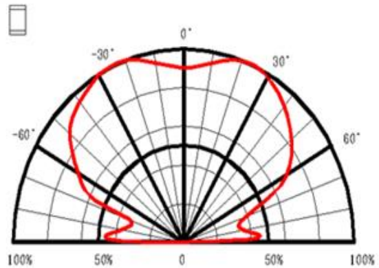
Directive Characteristics
