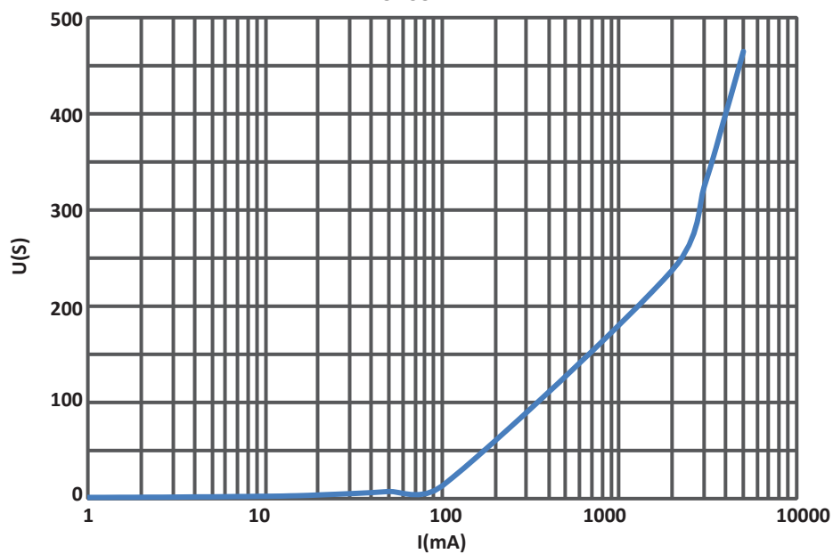
FIGURE 6 UI CURVE
