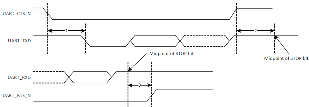
Figure 5: UART Timing
