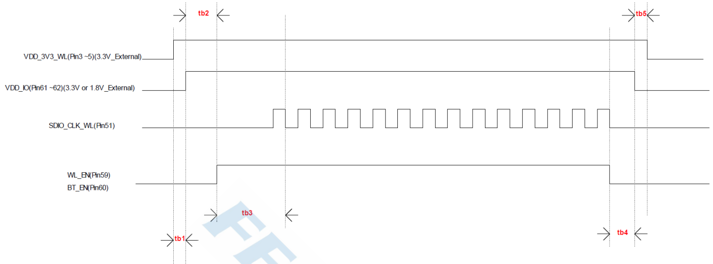
Figure 18: Power on and power off timing Sequence
