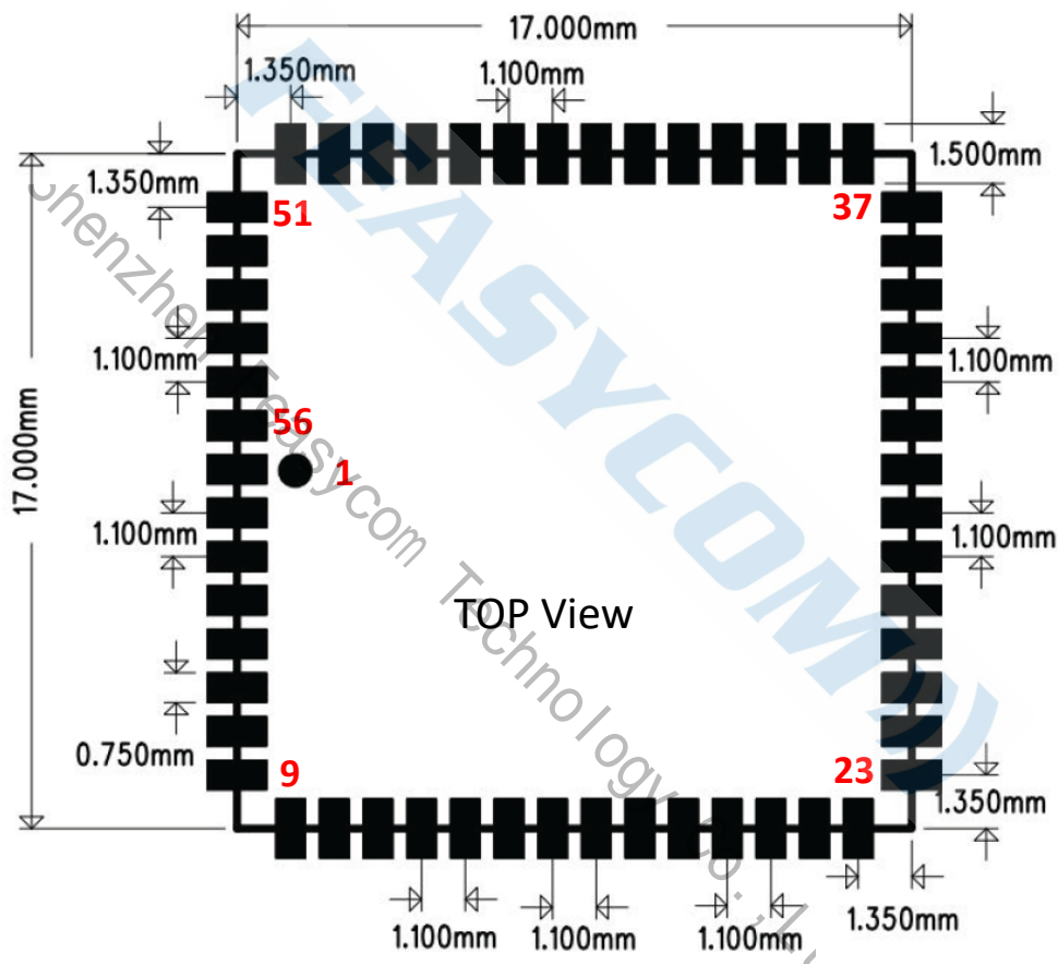
Figure 20: FSC-BW101 footprint Layout Guide (Top View)
