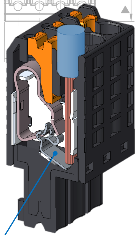
A weak push by wire activates the clamp
