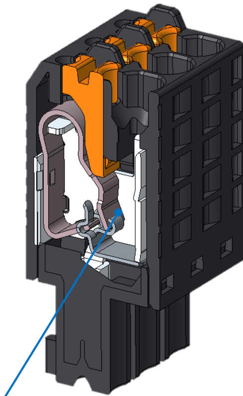
Clamping spring's delivered preloaded
