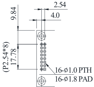
PIN DETAIL
