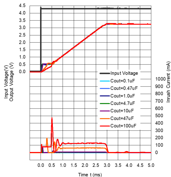
R1517x331E/F ( C_D = 10 \text{ nF} )
