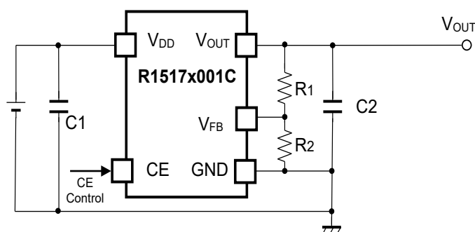
R1517x001C Typical Application
