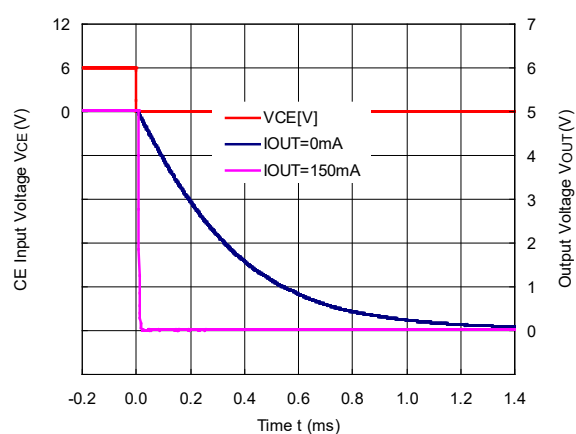
R1517x501F (C2 = 0.1 μF, CD = 1 nF)
