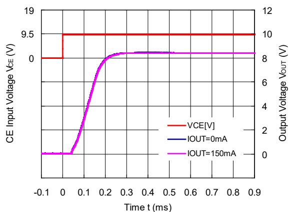
R1517x251E/F (C2 = 0.1 μF, C D = 1 nF)
