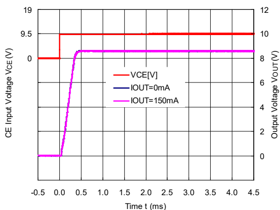
R1517x851E/F (C2 = 0.1 μF, CD = 1 nF)
