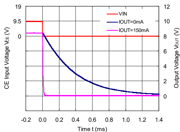
R1517x251F (C2 = 0.1 μF, C D = 1 nF)
