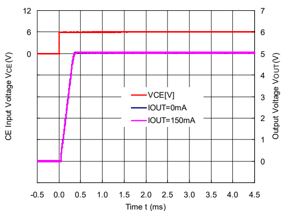
R1517x501E/F (C2 = 0.1 μF, CD = 1 nF)
