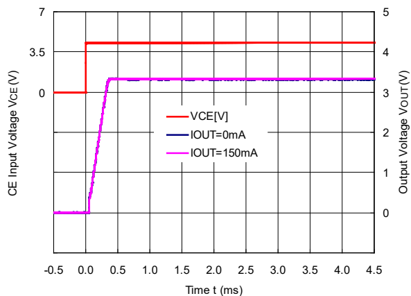
R1517x331E/F (C2 = 0.1 μF, CD = 1 nF)
