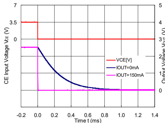
R1517x25xD (C2 = 0.1 \mu F)
