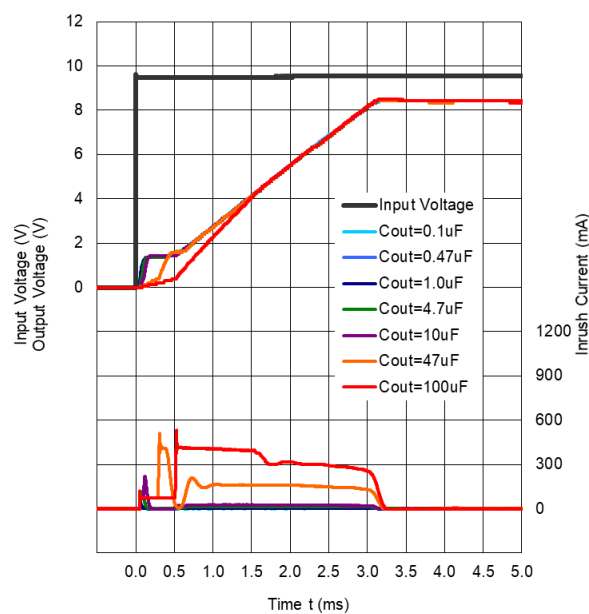
R1517x851E/F ( C_D = 10 \text{ nF} )
