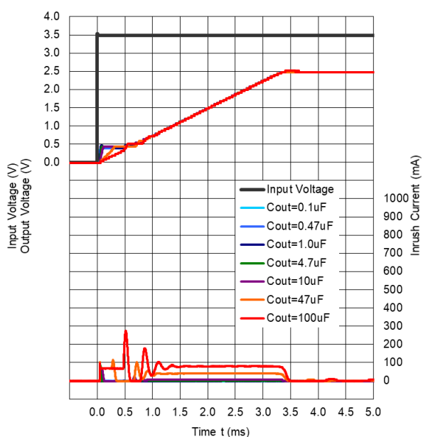
R1517x251E/F ( C_D = 10 \text{ nF} )
