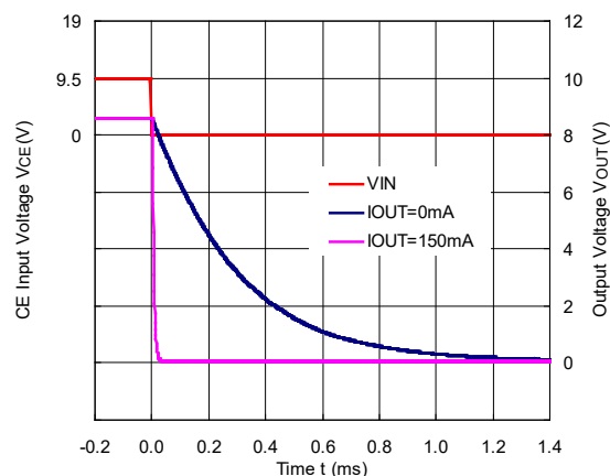
R1517x851F (C2 = 0.1 μF, CD = 1 nF)
