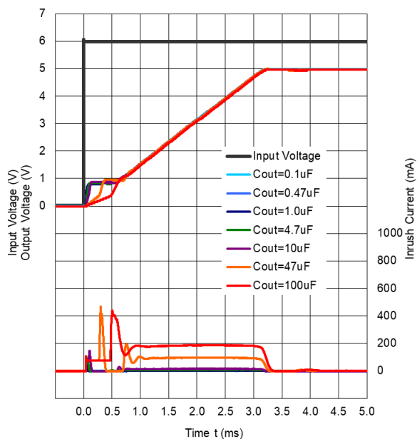
R1517x501E/F ( C_D = 10 \text{ nF} )
