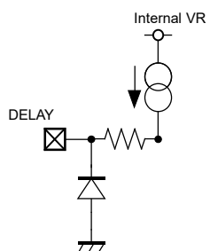
DELAY Pin (R1517xxx1E/F)
