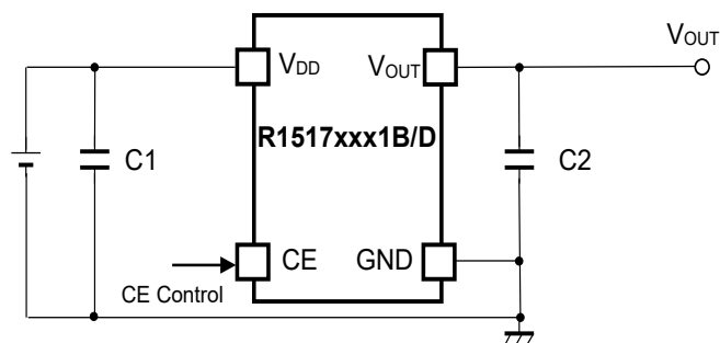
R1517xxx1B/D Typical Application
