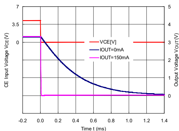
R1517x331F (C2 = 0.1 μF, CD = 1 nF)
