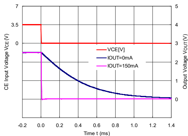
R1517x251F (C2 = 0.1 μF, C D = 1 nF)
