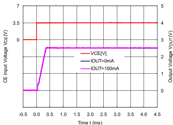
R1517x251E/F (C2 = 0.1 μF, C D = 1 nF)
