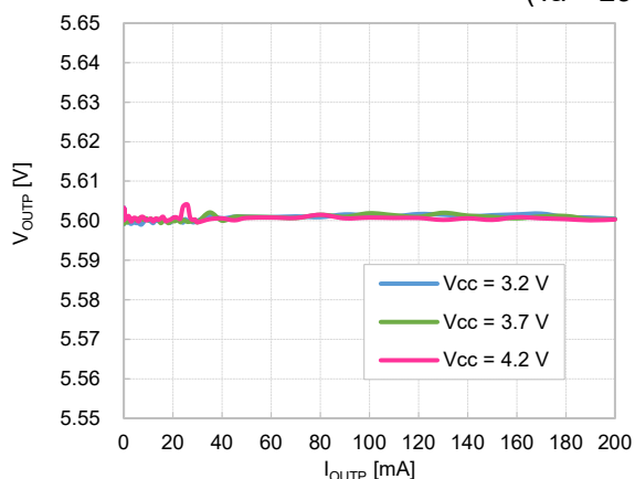
R1287x001B/F ( V_{OUTP} = 5.6\text{ V} ) ( T_a = 25^\circ\text{C} )
