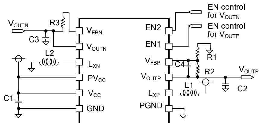
R1287x001y Typical Application (Adjustable Output Voltage Type)
