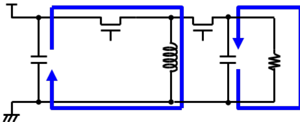
PMOSFET-ON (INVERTING)
