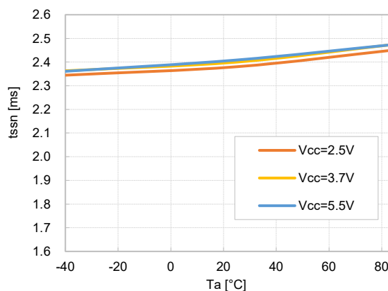
24) CH2 Soft-Start Time vs. Temperature R1287xxxxxy
