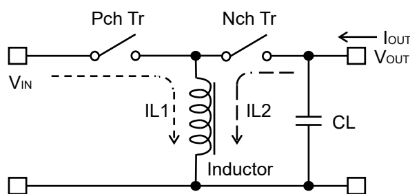
Basic Circuit
