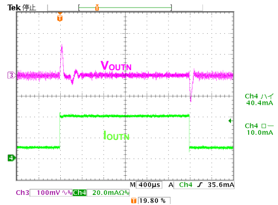
R1287x001B/F ( V_{OUTN} = -5.0\text{ V} ) ( T_a = 25^\circ\text{C} )
