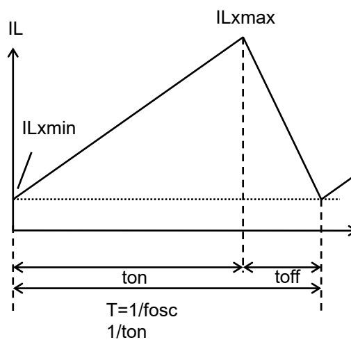
Inductor Current Waveshapes (IL) through Inductor (L)
