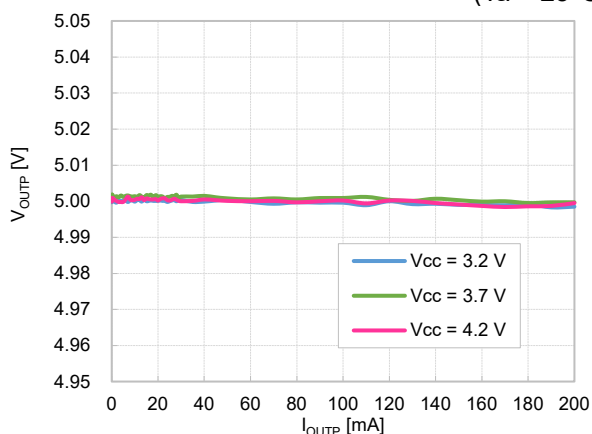
R1287x001D/H ( V_{OUTP} = 5.0\text{ V} ) ( T_a = 25^\circ\text{C} )
