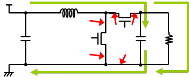
PMOSFET-ON (BOOST)
