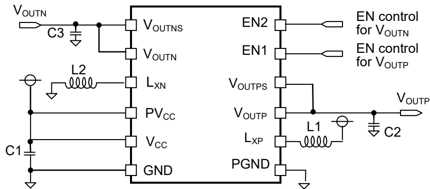
R1287xxxxy Typical Application (Fixed Output Voltage Type)
