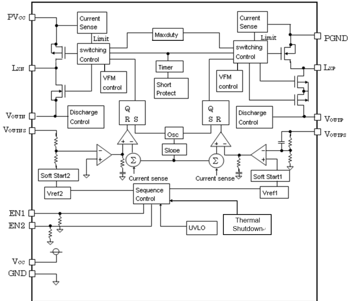
R1287xxxxxy Block Diagram (Fixed Output Voltage Type)
