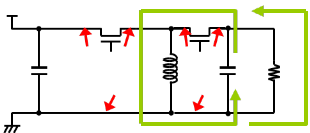
NMOSFET-ON (INVERTING)
