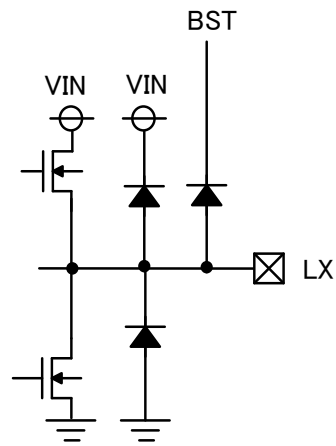
< LX Pin >
