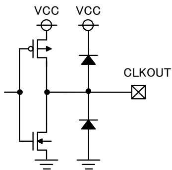
< CLKOUT Pin >
