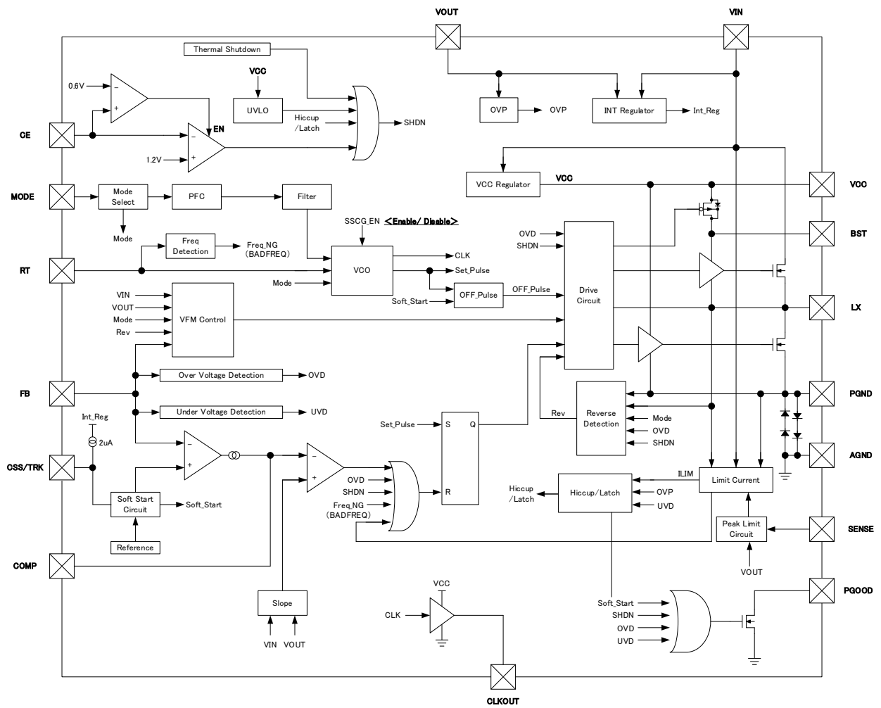
R1273LxxxA
