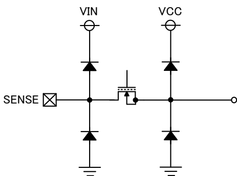
< SENSE Pin >
