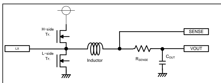
Figure A Detection with Sense Resistance
