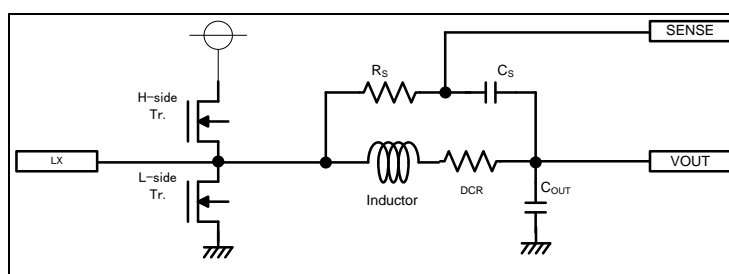
Figure B Detecting with Inductor's DCR
