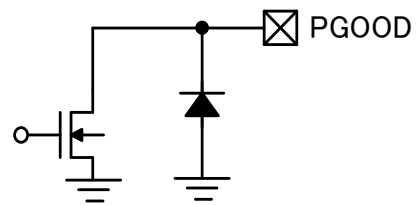
< PGOOD Pin >
