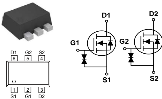
SOT-563 Pin Configuration
