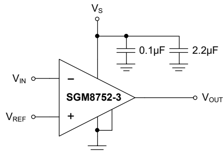
Figure 3. Recommended Connections for the SGM8752-3
