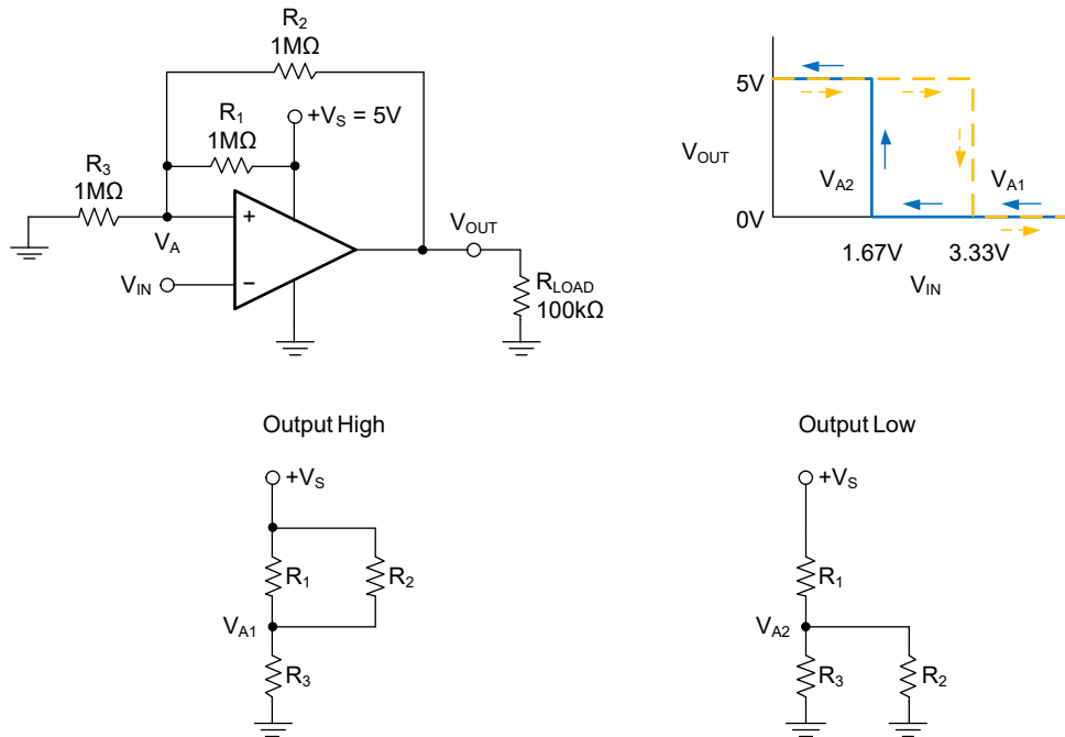
Figure 3. SGM8714A-1 in an Inverting Configuration with Hysteresis
