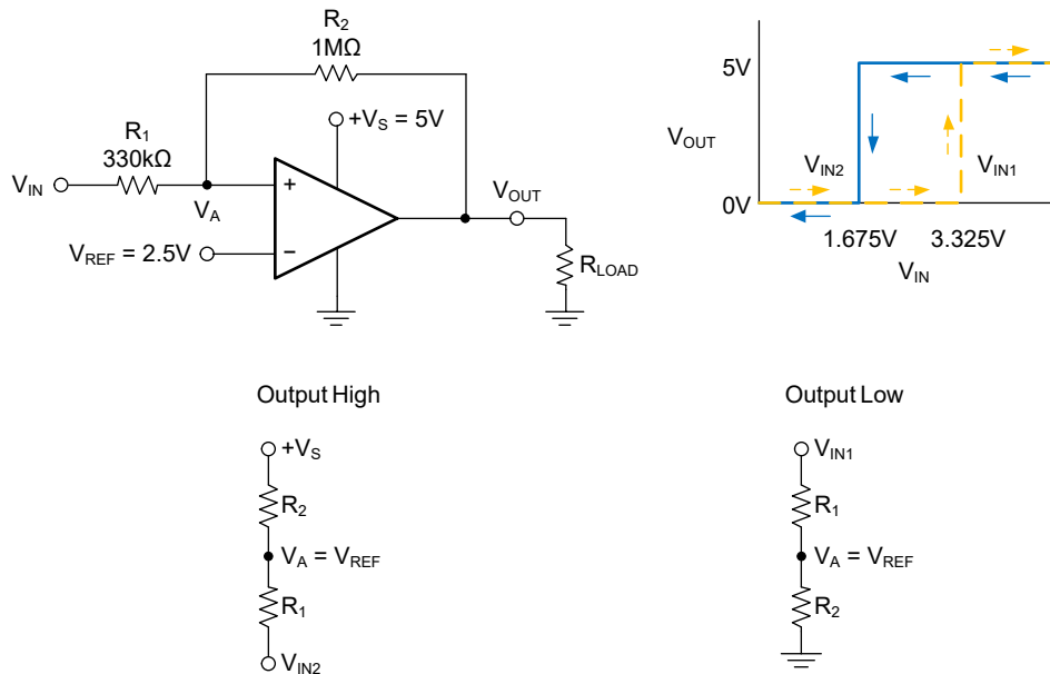
Figure 4. SGM8714A-1 in a Non-Inverting Configuration with Hysteresis
