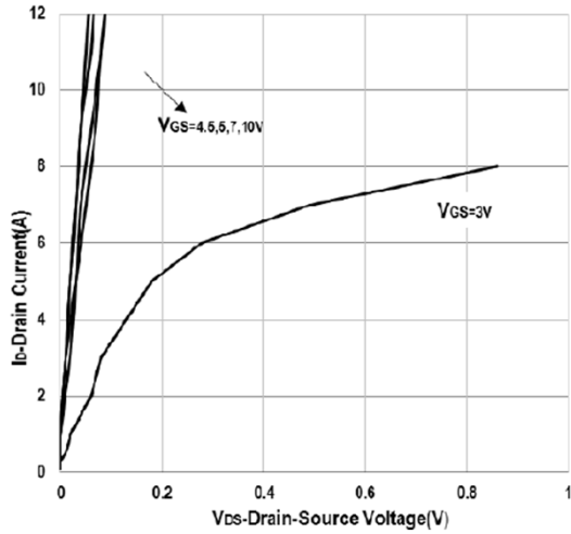
FIG.1-Typical Output Characteristics
