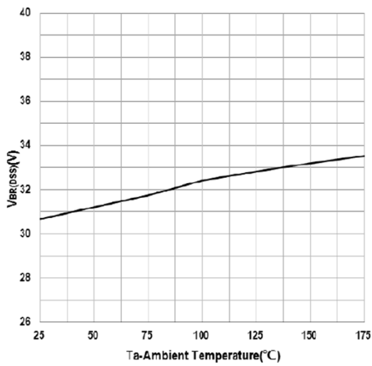
FIG.3-Drain-Source Breakdown Voltage vs. T_A
