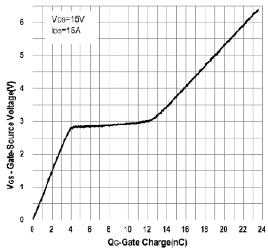
FIG.4-Gate Charge Characteristics
