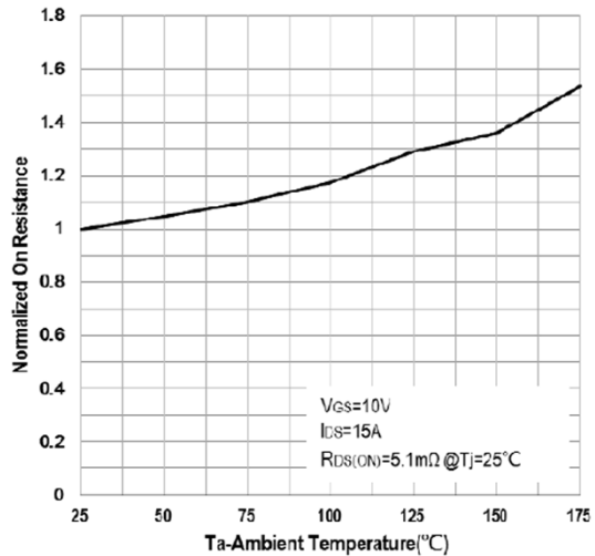
FIG.6-Normalized R_{DSON} vs. T_A
