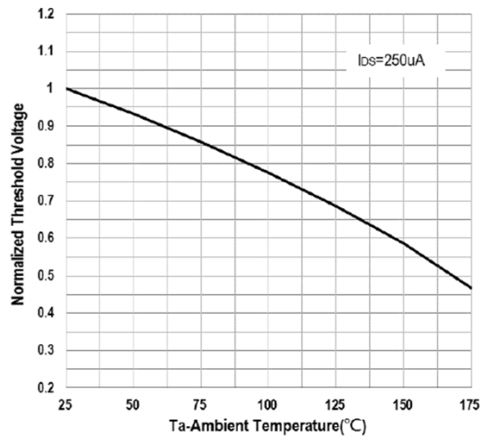
FIG.5-Normalized V_{GS(th)} vs. T_A
