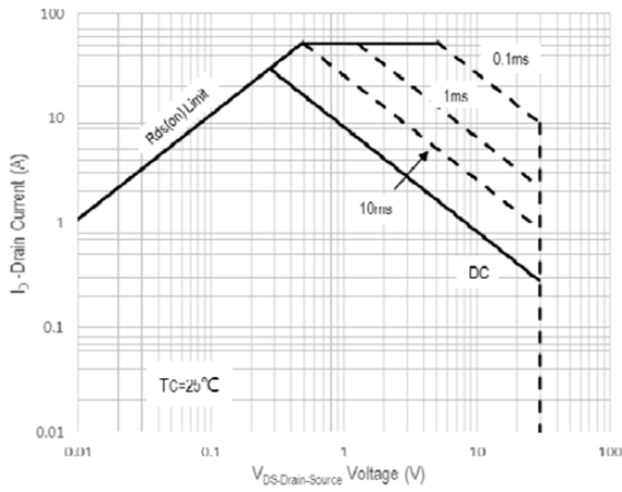
FIG.7-Safe Operating Area
