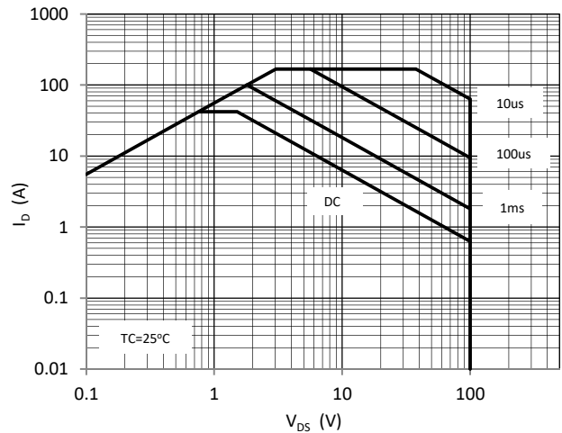
FIG. 6-Safe Operating Area
