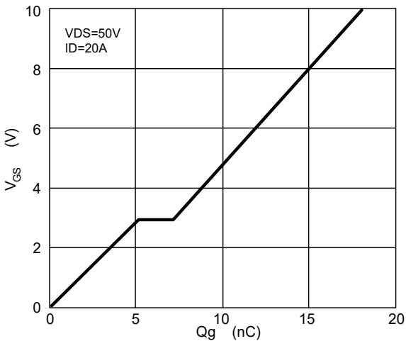
FIG. 5-Gate Charge Characteristics
