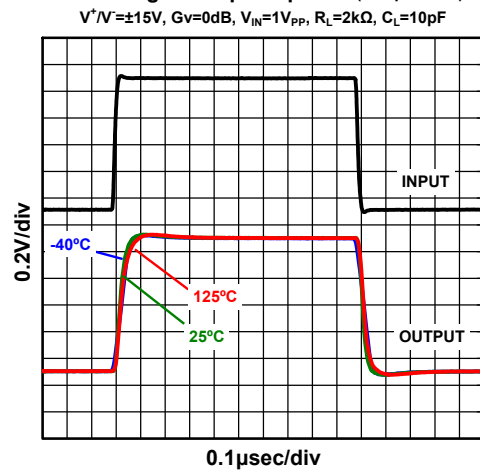
Small-Signal Step Response (Temperature)
