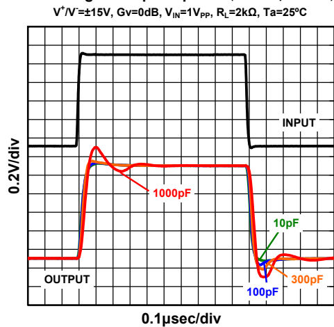
Small-Signal Step Response (Load Capacitance)
