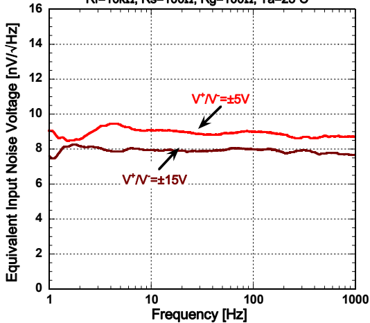
Equivalent Input Noise Voltage
