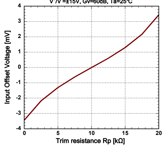
Input Offset Voltage vs. Trim Resistance
