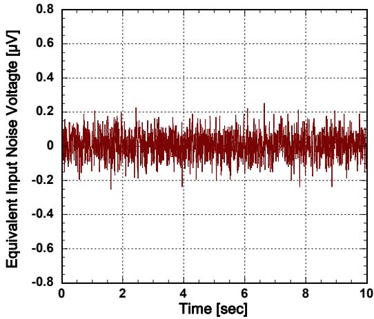
Equivalent Input Noise Voltage
