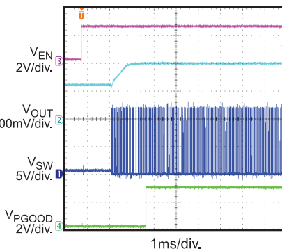
Pre-Bias Start-Up
