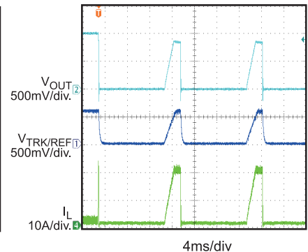
Over-Current
