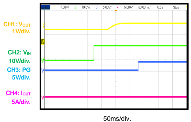
Pre-Biased Start-Up
