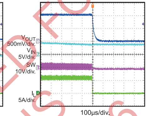
Shutdown Through V_{IN} I_{OUT} = 6A
