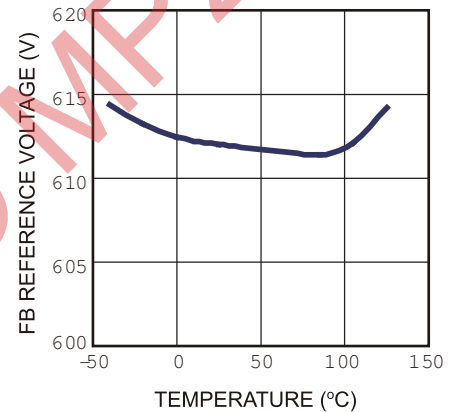
FB Reference Voltage vs. Temperature
