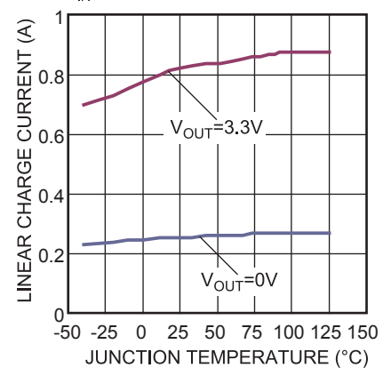
Linear Charge Current vs. Junction Temperature V_{IN}=4.2V
