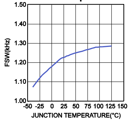
F sw vs. Junction Temperature
