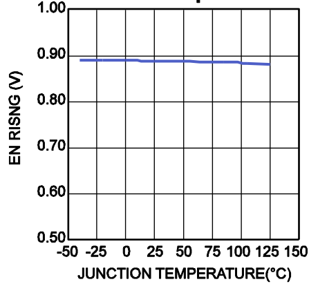
EN Rising vs. Junction Temperature
