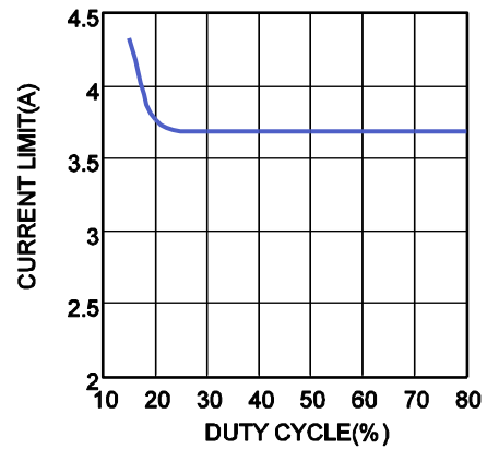
Current limit vs. Duty
