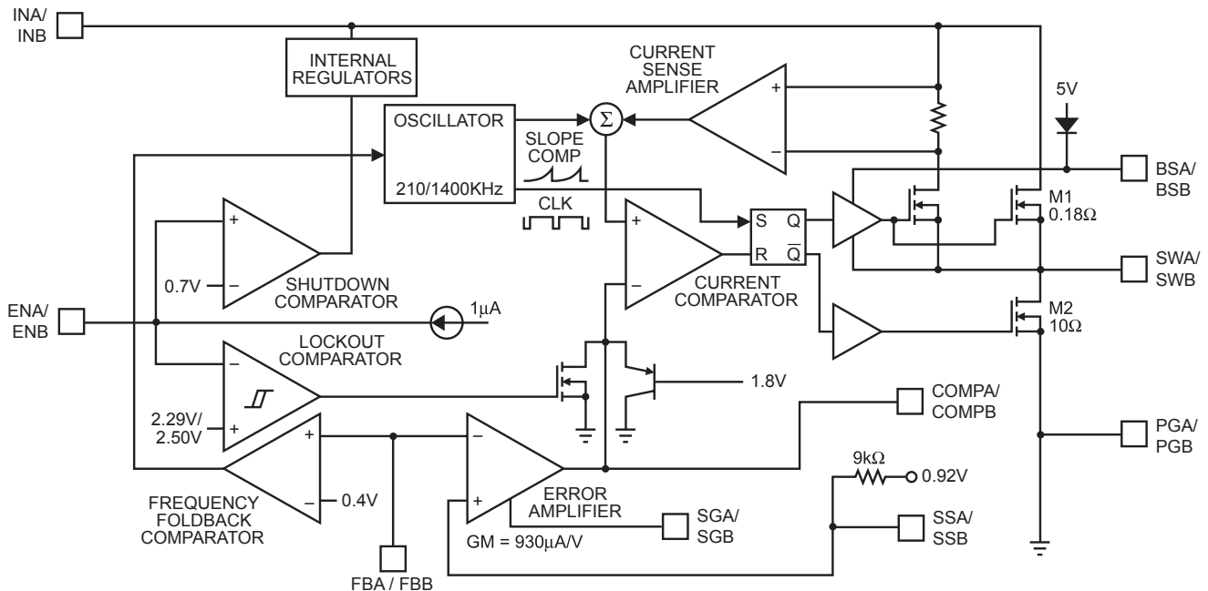
Figure 1—Functional Block Diagram (Diagram portrays 1/2 of the MP29373)
