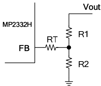
Figure 4: Feedback Network
