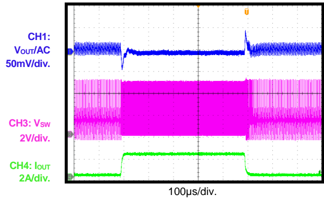
Load Transient
