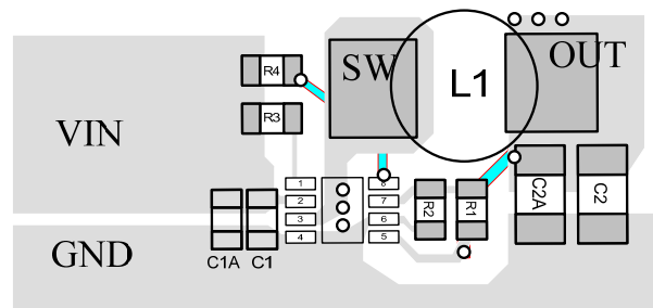
Figure 3: Layout Recommendation
