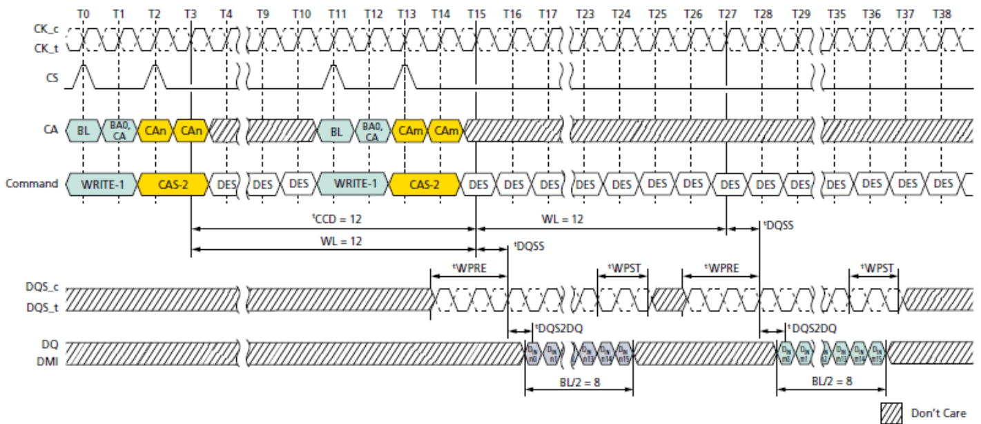
Consecutive WRITE: t^{\text{CCD}} = \text{MIN} + 4 , 1.5n\text{CK} Postamble
