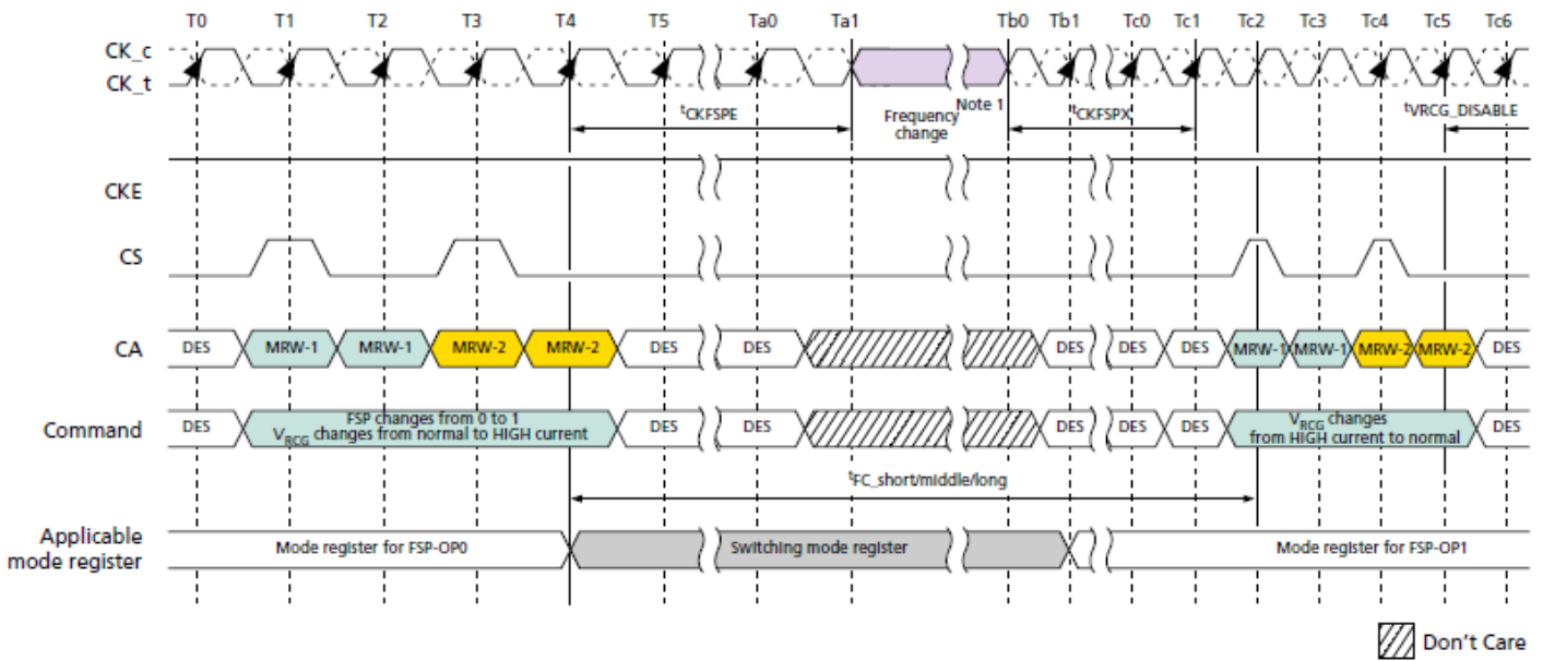
Frequency Set Point Switching Timing
