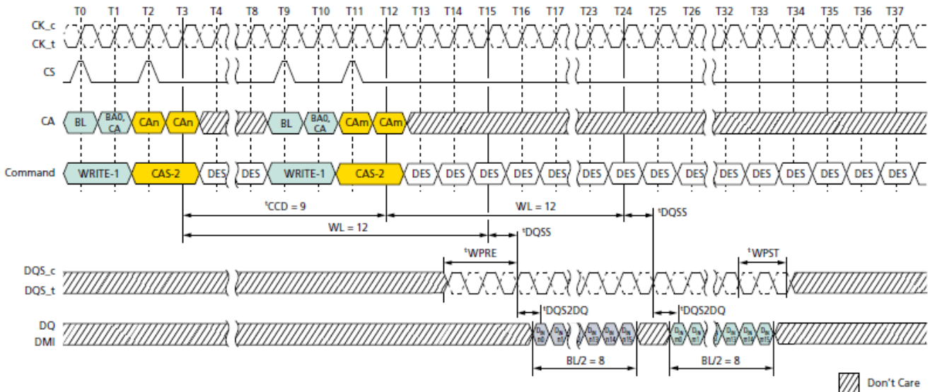
Consecutive WRITE: t'CCD = MIN + 1, 1.5nCK Postamble
