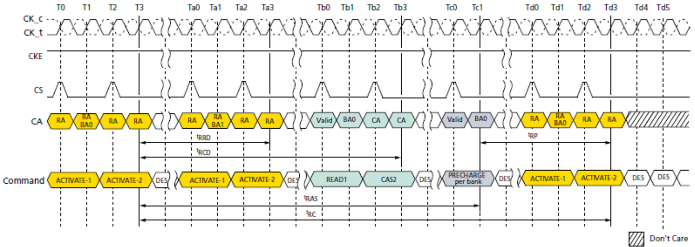
ACTIVATE Command
