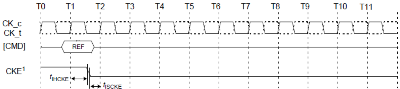
REFRESH Command to Power-Down Entry
