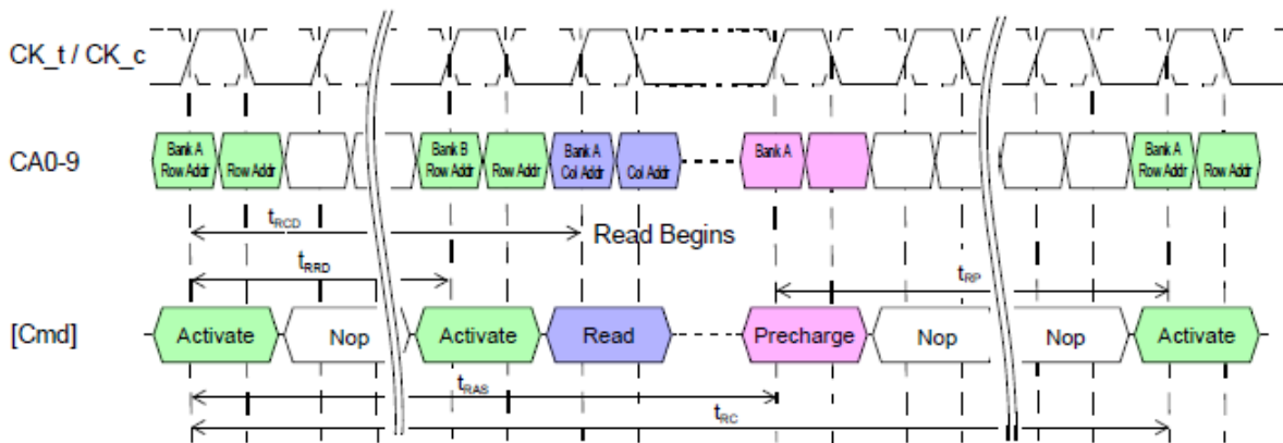
ACTIVATE Command
