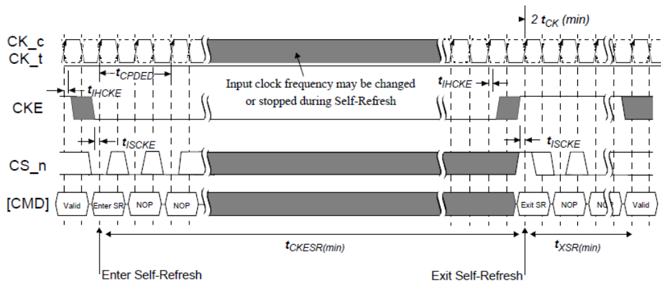
Self-Refresh Operation
