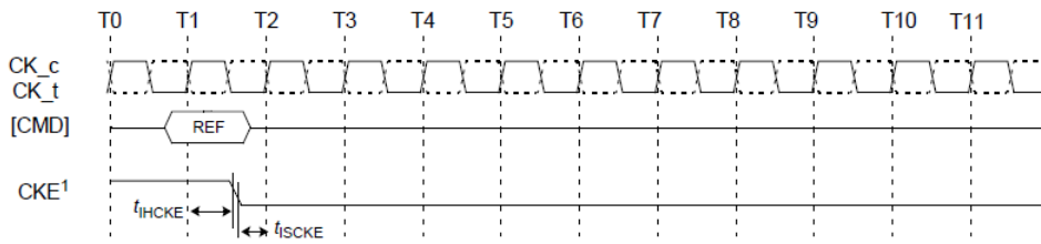
REFRESH Command to Power-Down Entry
