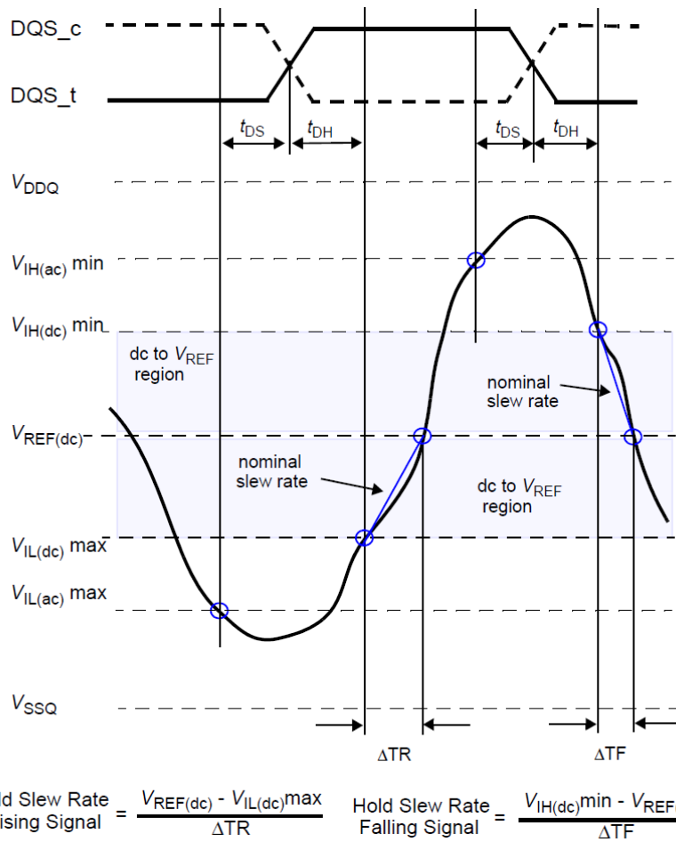
Illustration of nominal slew rate for hold time t_{DH} for DQ with respect to strobe
