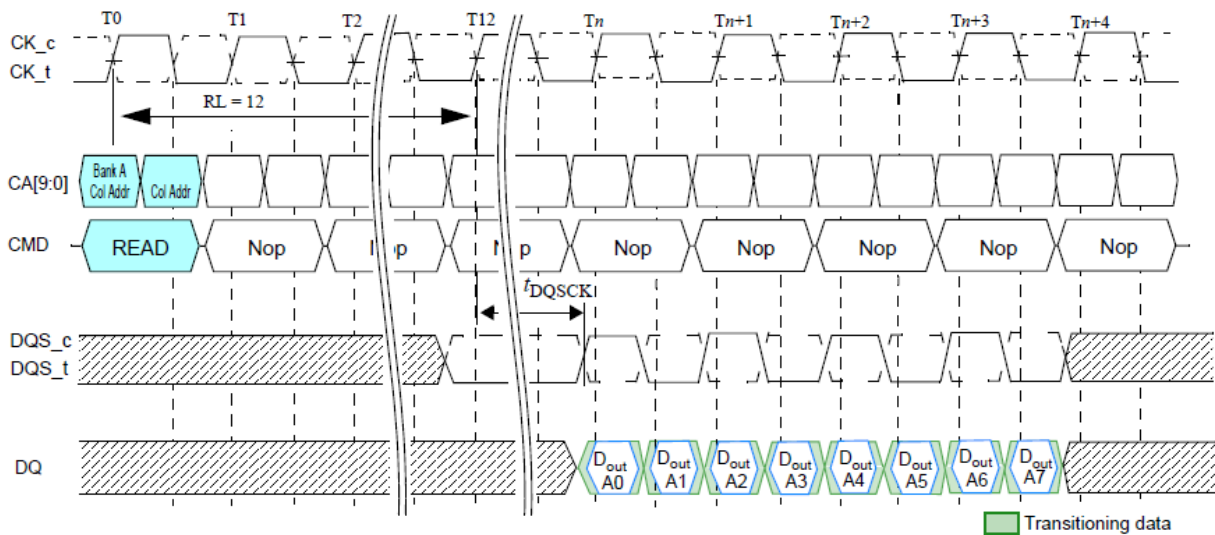
Burst Read: RL = 12, BL = 8, t_{DQSCk} < t_{ck}
