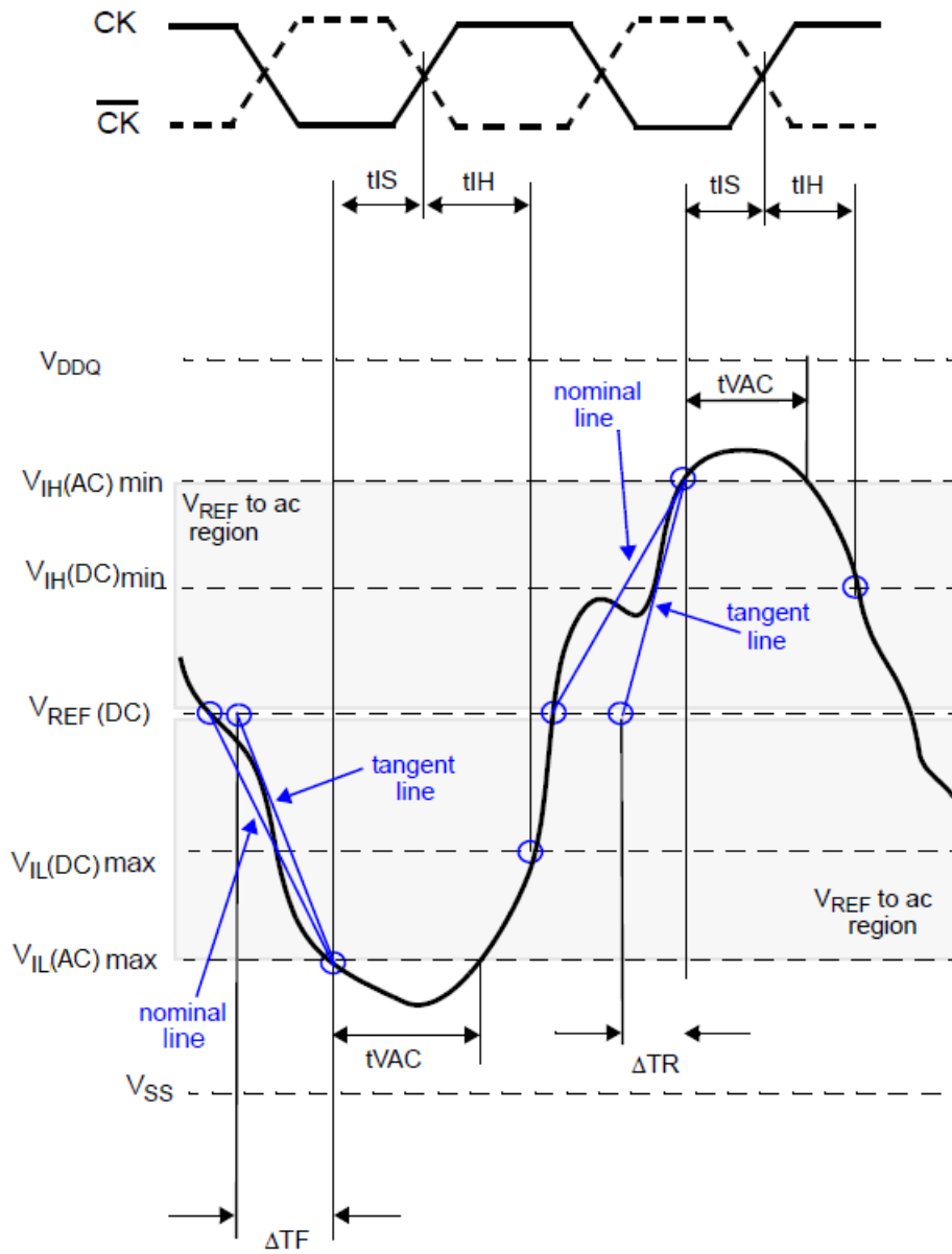
Illustration of tangent line for setup time tIS (for ADD/CMD with respect to clock)
