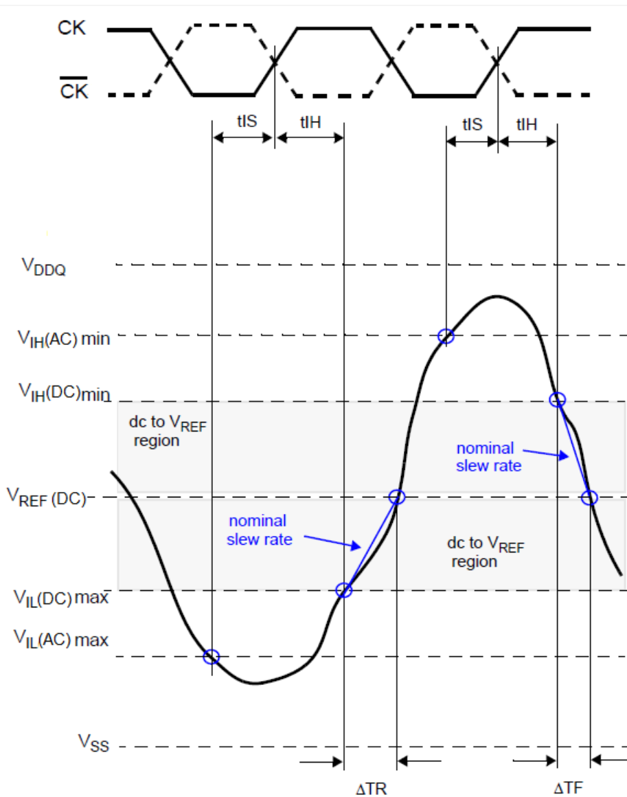
Illustration of nominal slew rate for hold time t H (for ADD/CMD with respect to clock)
