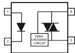
Pin Configuration
