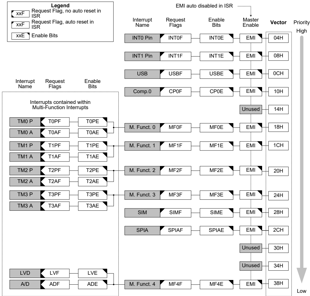
Interrupt Structure – HT66FB542
