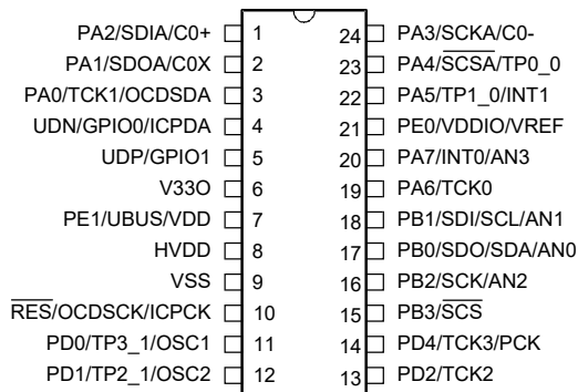
HT66FB542/HT66VB542 24 SSOP-A
