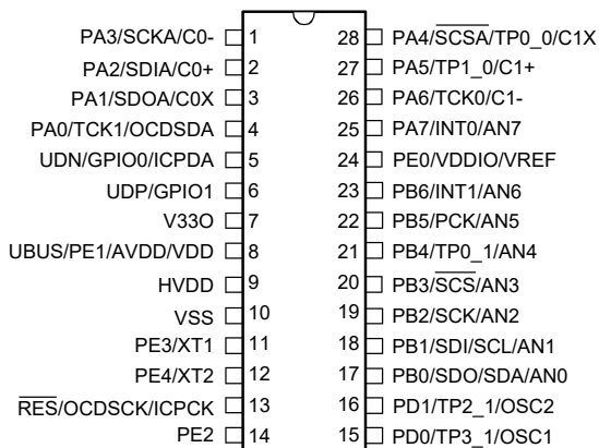
HT66FB550/HT66VB550 28 SSOP-A
