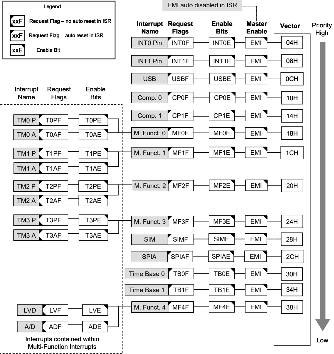
Interrupt Structure – HT66FB540/HT66FB550/HT66FB560
