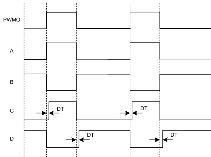
Dead Time Insertion Timing
