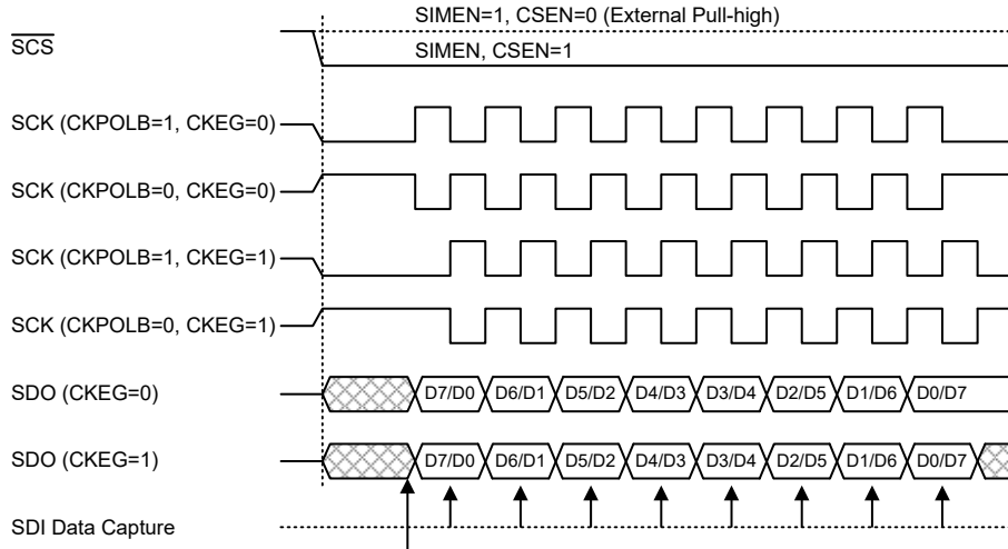
Write to SIMD SPI Master Mode Timing
