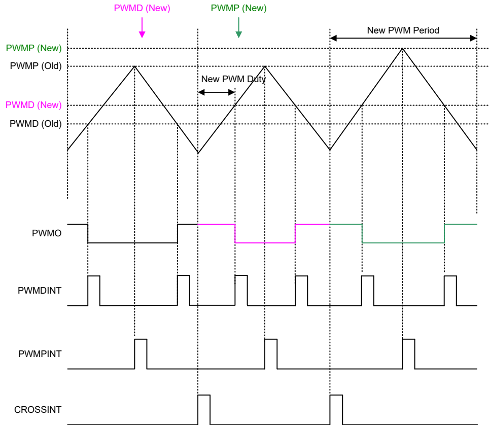
PWM Center-Aligned Mode Timing Diagram
