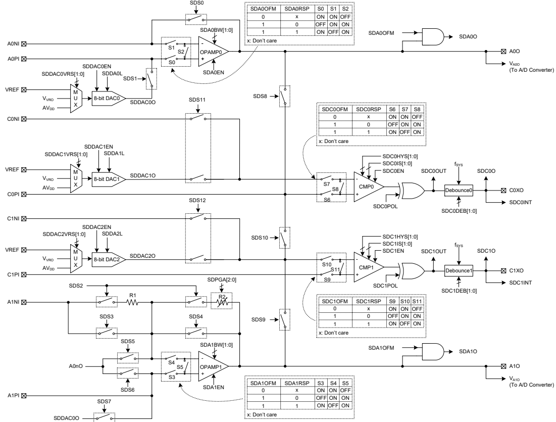
Internal Analog Function Block Diagram
