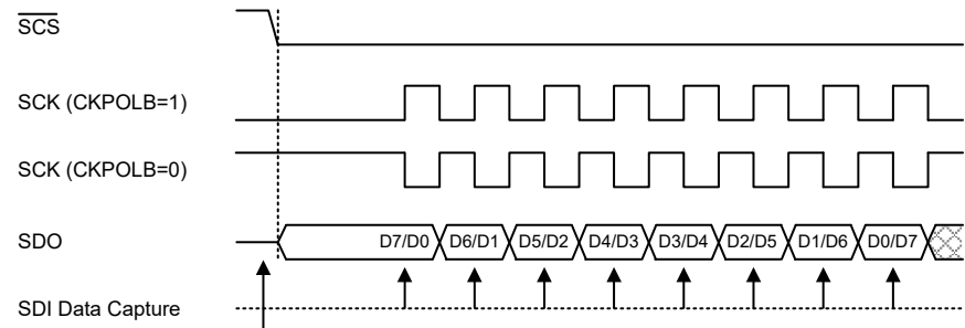
Write to SIMD (SDO changes as soon as writing occurs; SDO is floating if \overline{SCS}=1 )
