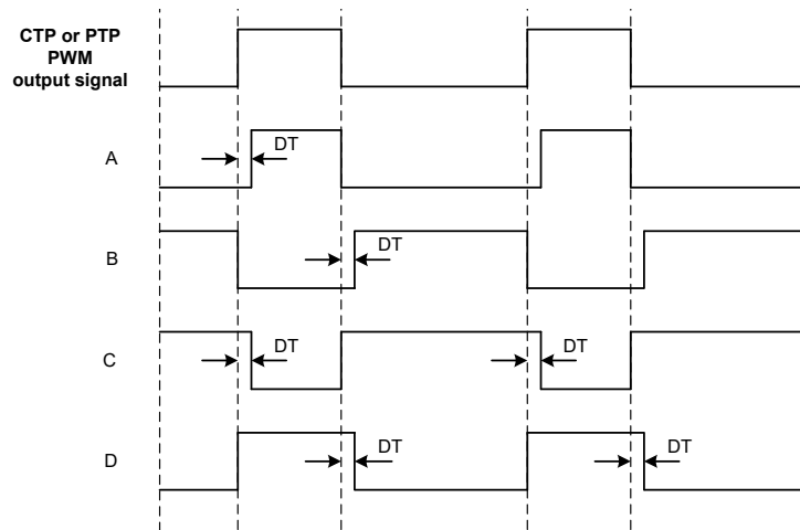
Complementary PWM Output with Dead Time Control
