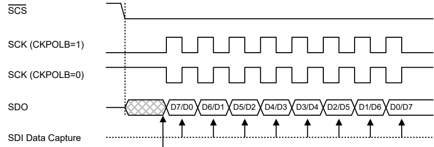
Write to SIMD (SDO does not change until first SCK edge)
