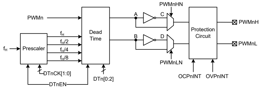
Complementary PWM Output with Dead Time Block Diagram (n=0~1)
