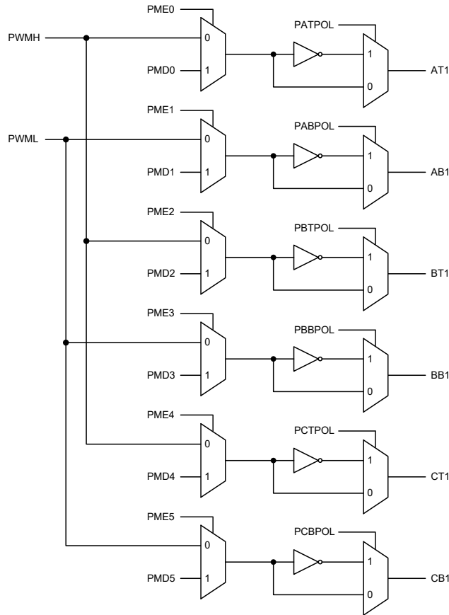
Mask Circuit Block Diagram
