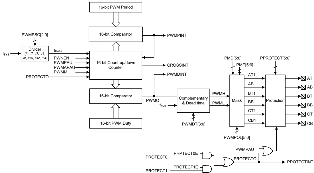
16-bit Enhanced PWM Control Circuit Block Diagram
