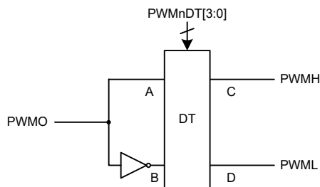
Complementary PWM Output with Dead Time Control
