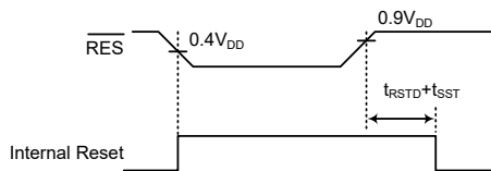
RES Reset Timing Chart
