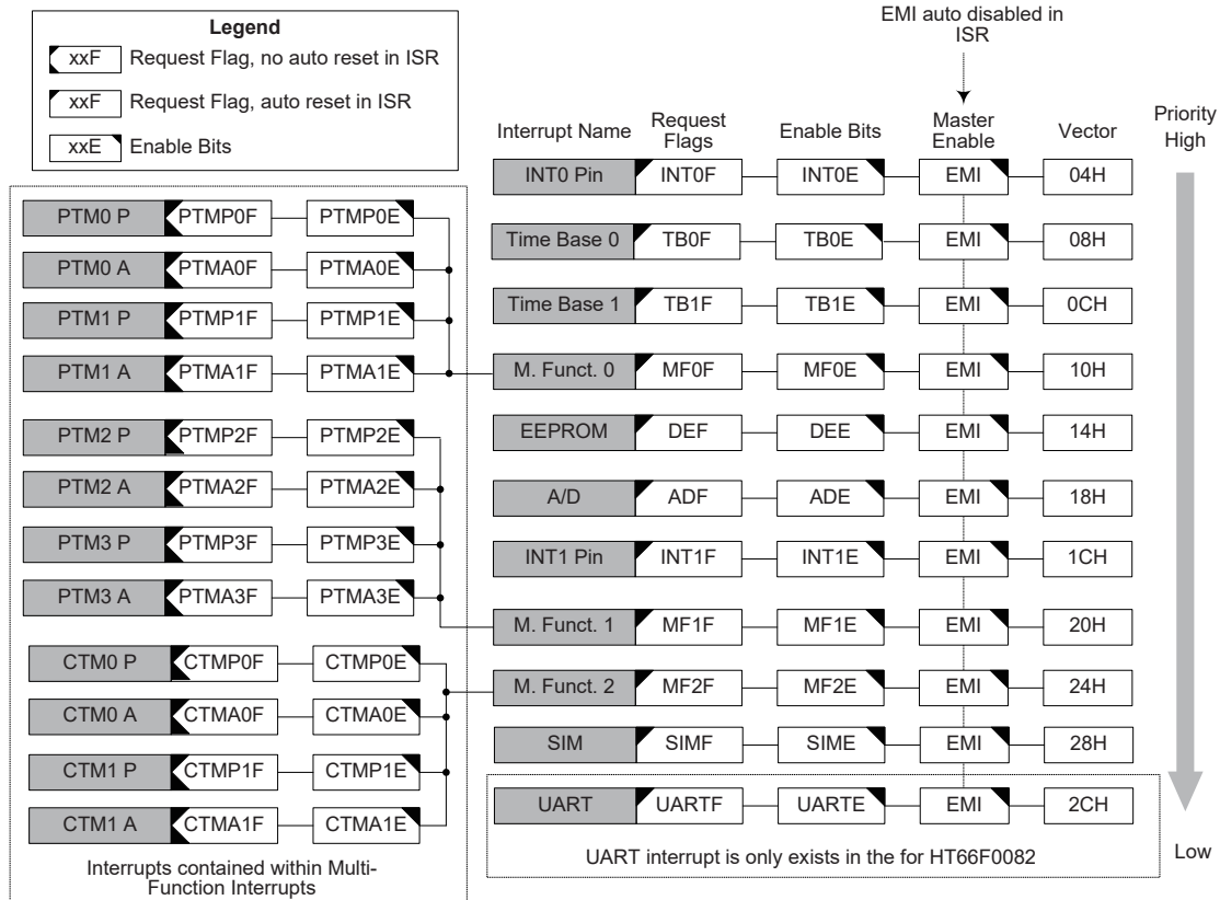
Interrupt Structure
