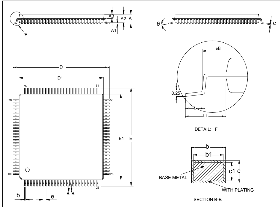
Figure 5-5. LQFP100 package outline
