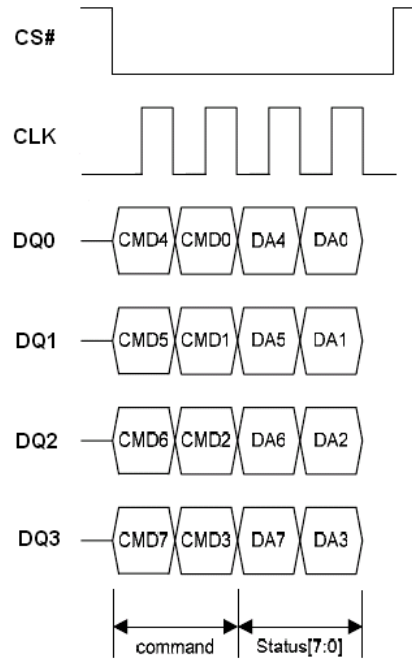
Figure 22. Write Status Register Instruction Sequence in QPI Mode
