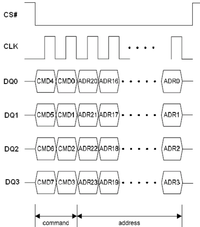
Figure 77. Block/Sector Erase Instruction Sequence in QPI Mode
